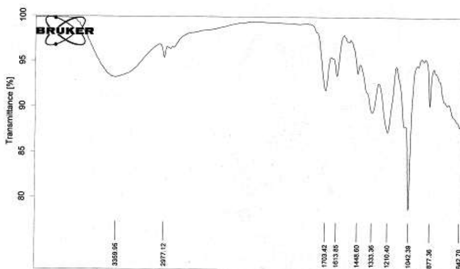
Fig-3: FT-IR spectrum of Terminalia chebula
