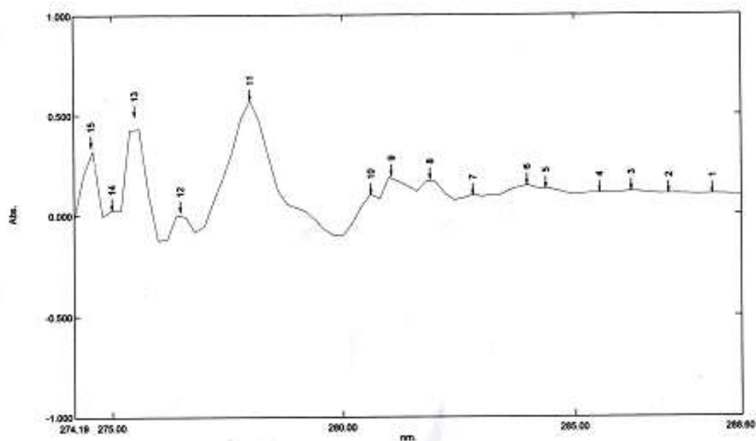
Fig-2: UV spectrum of ethanolic seed extract of Terminalia chebula
