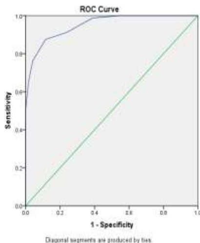
Area under the Curve Test Results Variables(s): SOFA score T0
