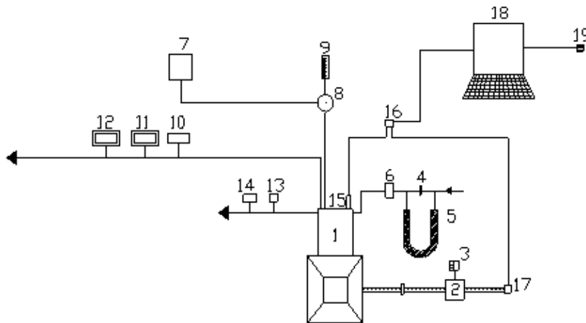
Figure 1. Experimental Set-up
