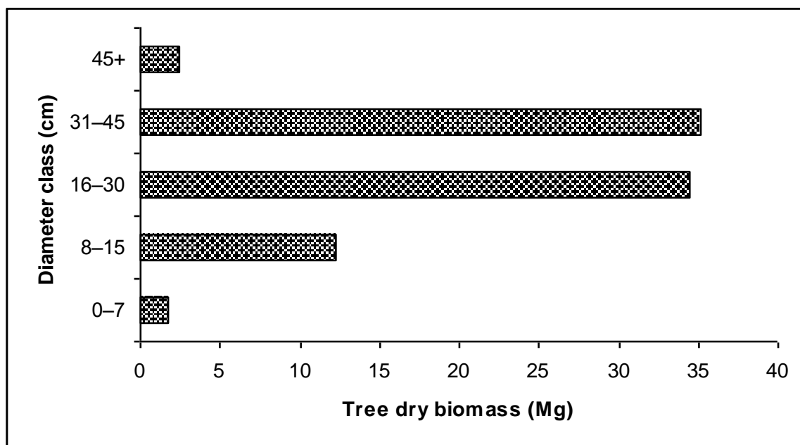
Fig. 1. Contribution of DBH classes to total dry biomass in Cooum river bank, Chennai, India.
