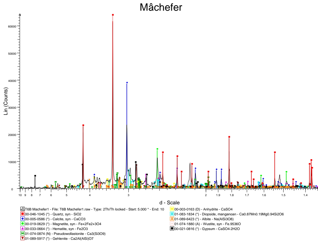
Fig-2: Analysis by X-Rays Diffraction
