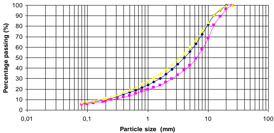
Fig-1: Particle size distribution by sieving
